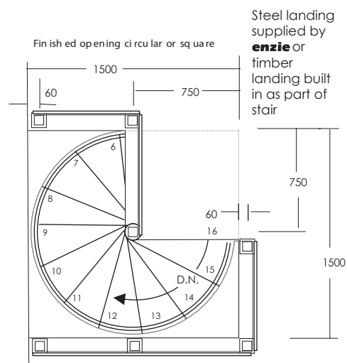
Standard stairwell and Balcony rails
