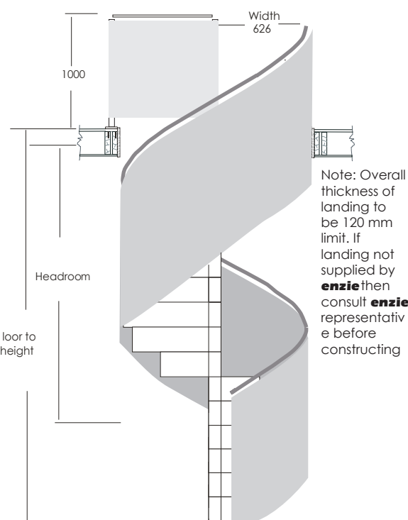
Standard stairwell and Balcony rails
