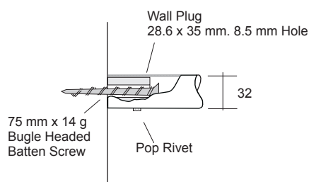
Wall fixing
