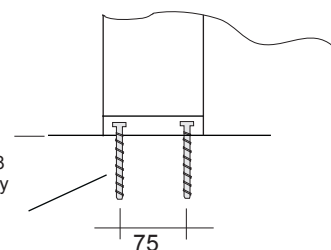
Concealed Base Plate
